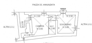
PIANO TERRA
