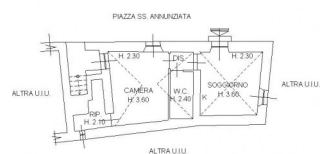
PIANO TERRA
