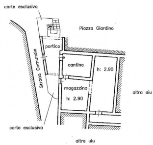
PIANO TERRENO
